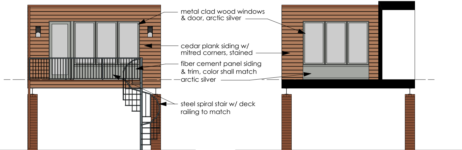
Partial East Elevation Scale: 1/8" = 1'-0"
