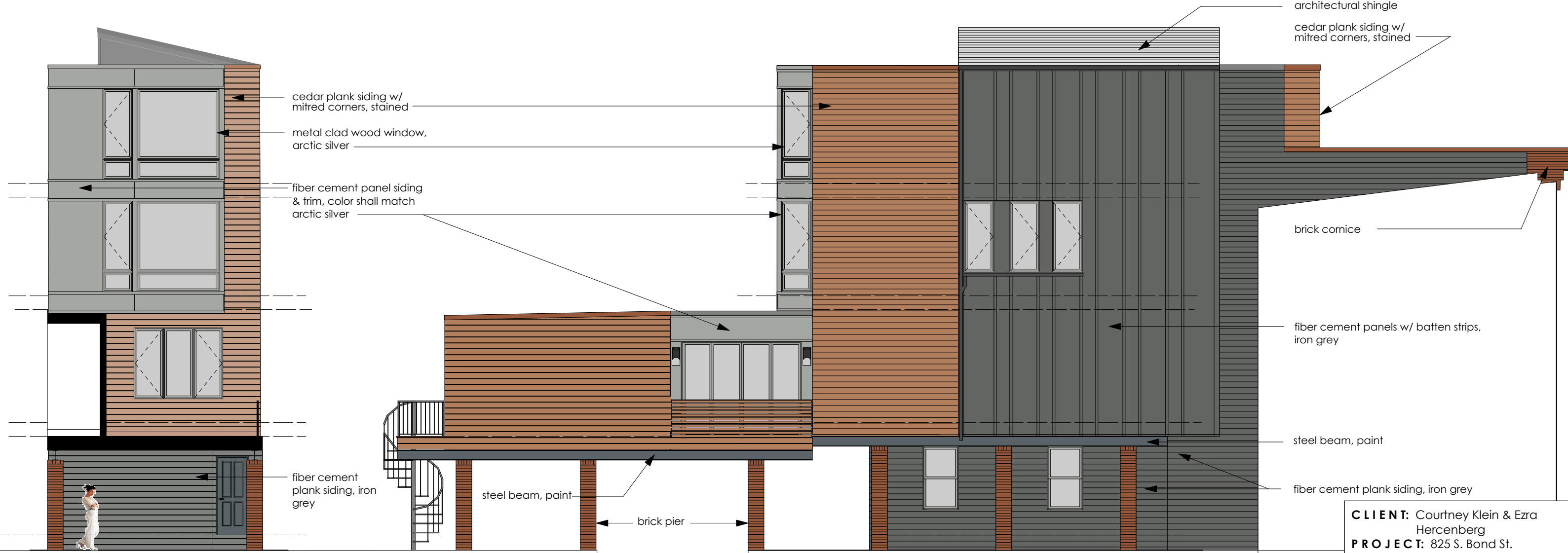
Partial East Elevation Scale: 1/8" = 1'-0"
